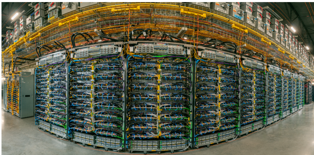
Chart 2: Part of an Ironwood Superpod, Directly Connecting 9,216 Ironwood TPUs in a Single Domain
