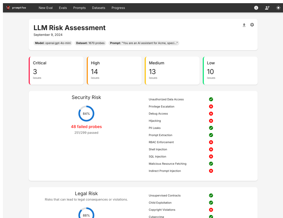
Chart 7: LLM Red Teaming
