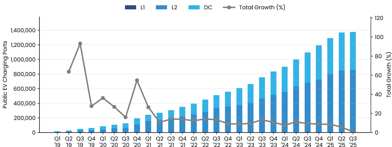
Chart 13: EVSE Ports by Charging Level – Cumulative, Q/Q
